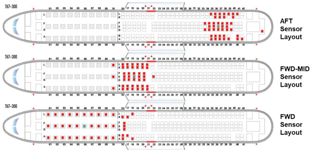
Figure 5. IBAC sensor layouts for each airframe and section tested. A single release seat is shown, but releases were done in multiple seats within a given row.
